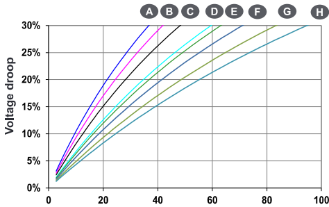
Locked rotor kVA at PF : 0.9
