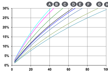
Locked rotor kVA at PF : 0.9
