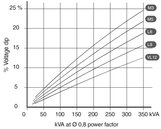
Load application (AREP or PMG excitation)
