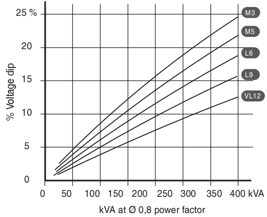
Load application (AREP or PMG excitation)
