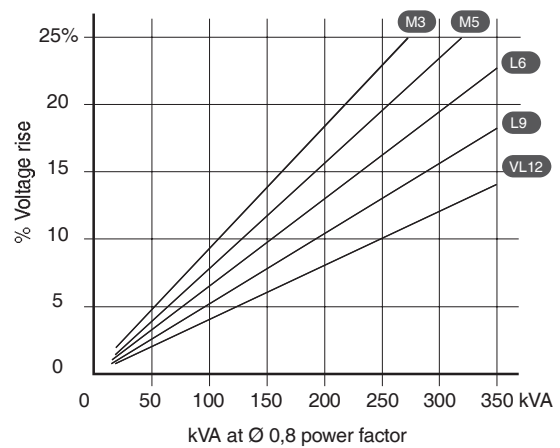
Load rejection (AREP or PMG excitation)
